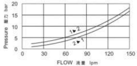
Pressure Drop 壓力降
